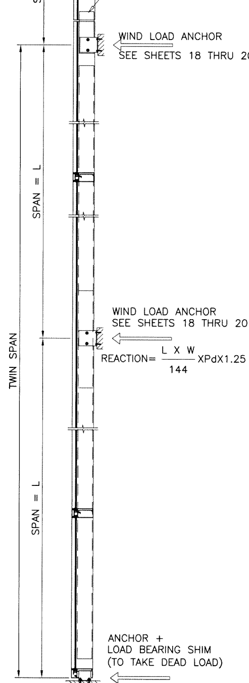
MULTIPLE SPANS
