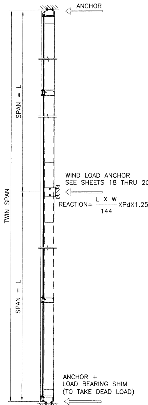
TWO SPAN
