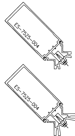
CORNER MULLION
