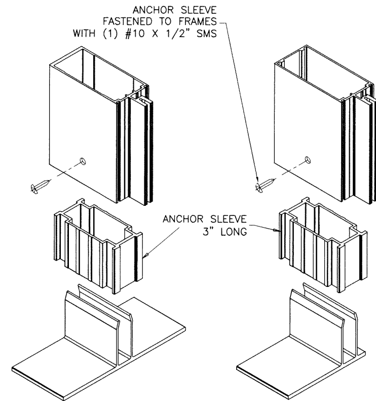
MULLION ANCHOR CLIP DETAIL '2'
