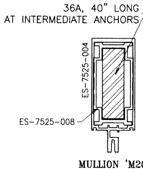
MULLION 'M2C'
